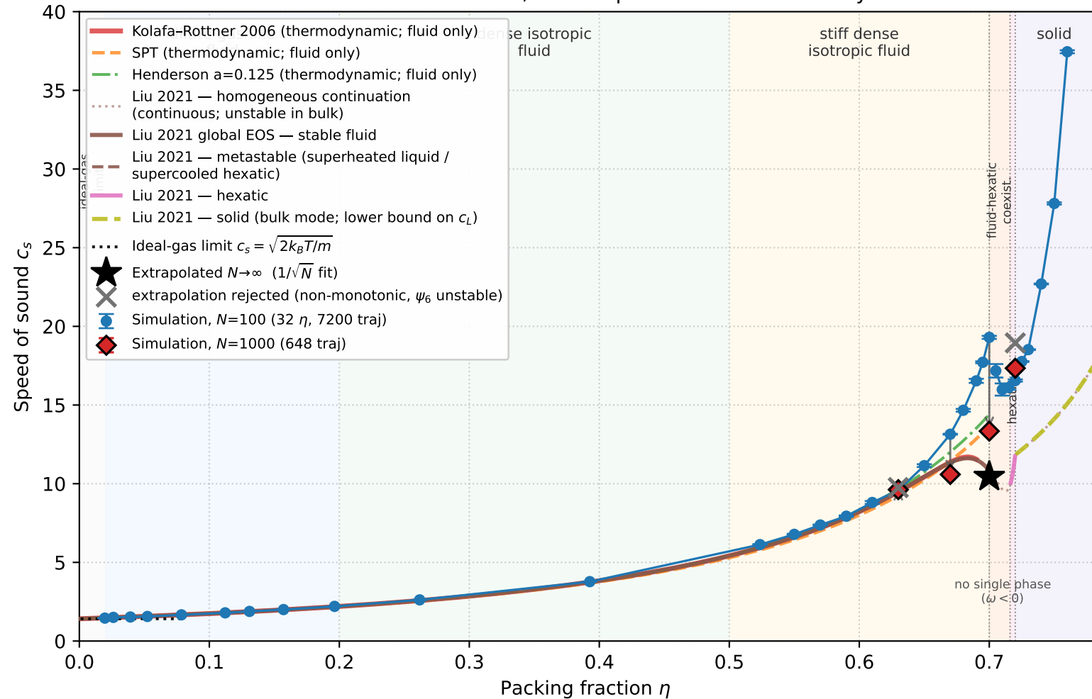
Hard-disk speed of sound: the high-density excess is finite-size arrows show N=100 \rightarrow N=1000 ; ★ extrapolates to the thermodynamic limit
